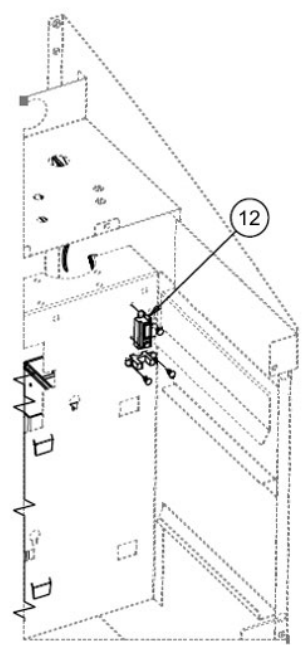
FRONT VIEW (CLIPPED)
